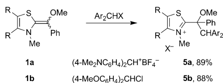
Scheme 6. Reactions of 1a,b with diarylcarbenium ions.
